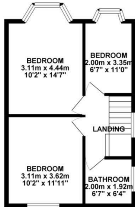
1ST FLOOR 39.23 sq. m. ( 422.31 sq. ft. )
