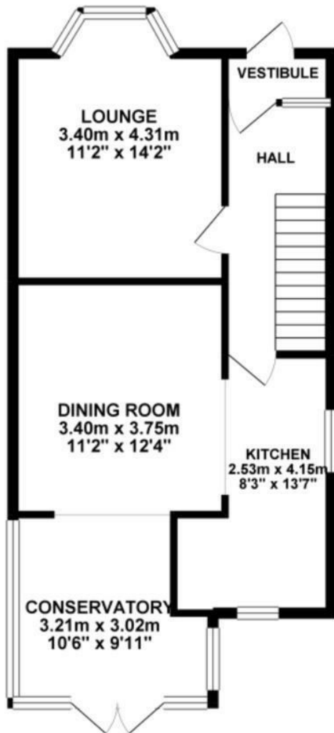
GROUND FLOOR 51.54 sq. m. ( 554.76 sq. ft. )
